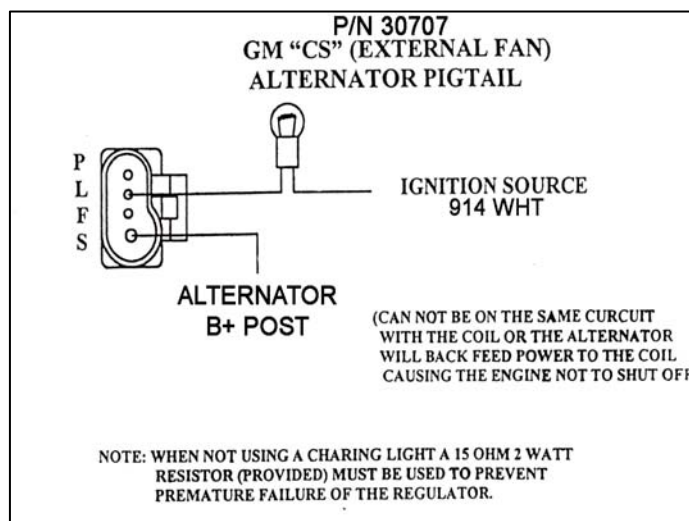
Figure 7-2D CS-130 Connector and Pin Out
